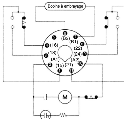
H2C(-F)R/H2C-SR
